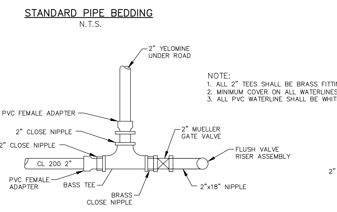
FLUSH VALVE DETAIL ON 2" LINE IN CUL DE SAC N.T.S.
