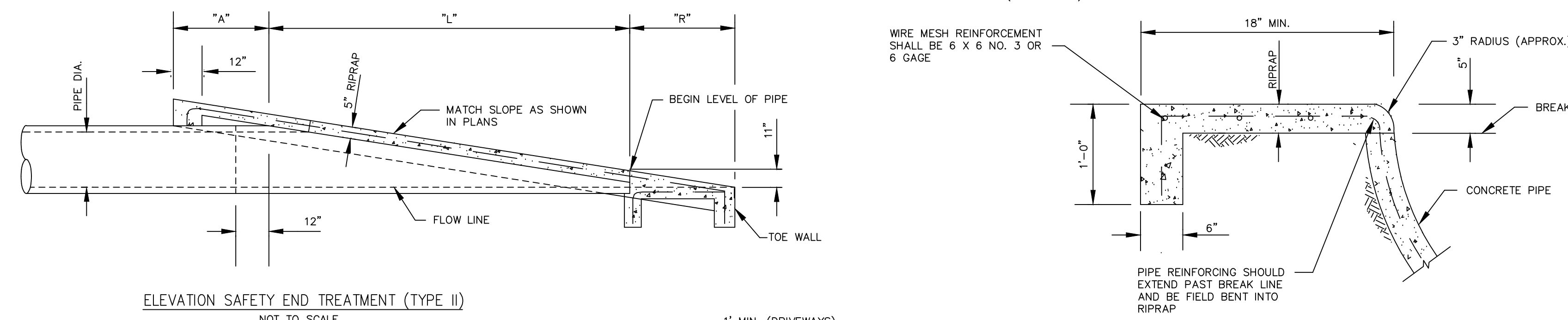
SECTION B-B
