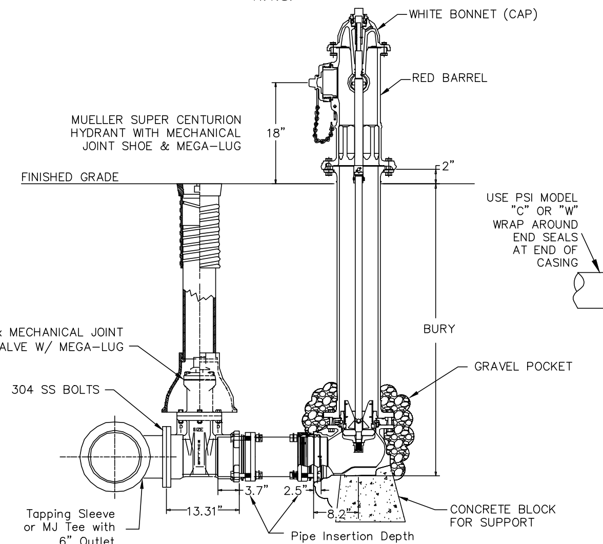
FIRE HYDRANT ASSEMBLY N.T.S.
