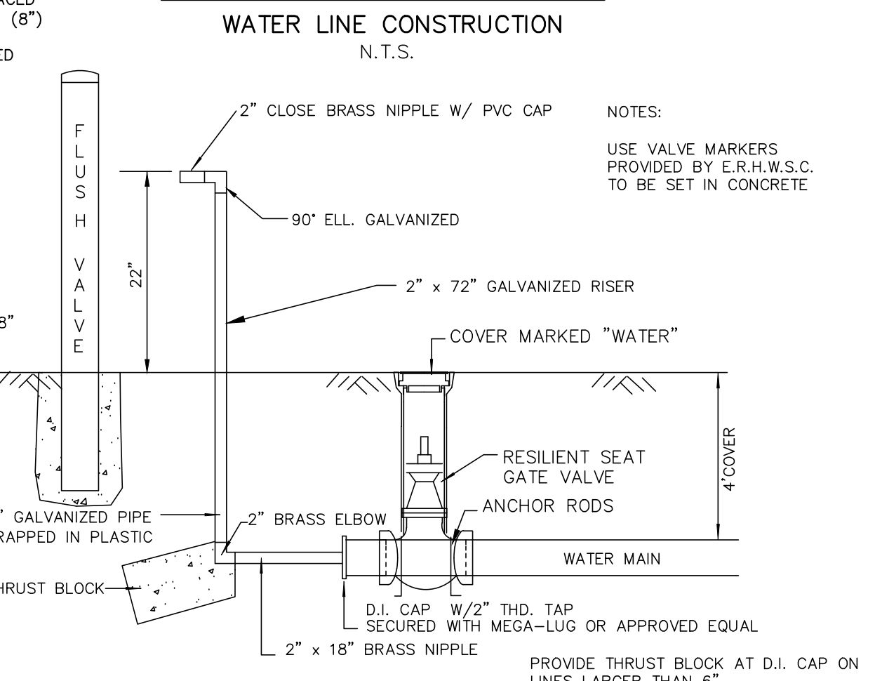
FLUSH VALVE ON FULL SIZE LINE VALVE DETAIL WATER LINE CONSTRUCTION N.T.S.
